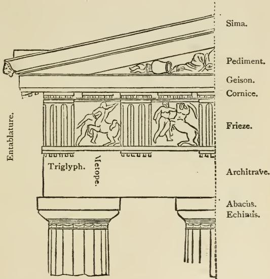
FIG. 40.—FROM THE PARTHENON, ATHENS.
